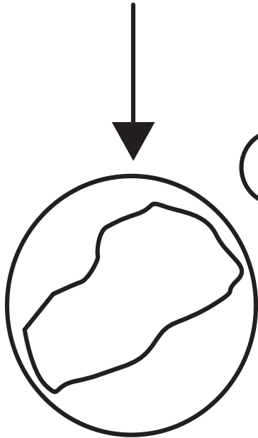
Asteroid
