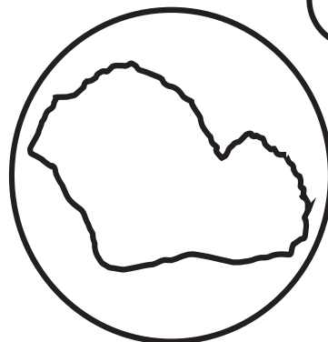
Comet
